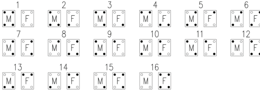
1109660 KILAVUZ KODLAMA PİMİ 16-72
