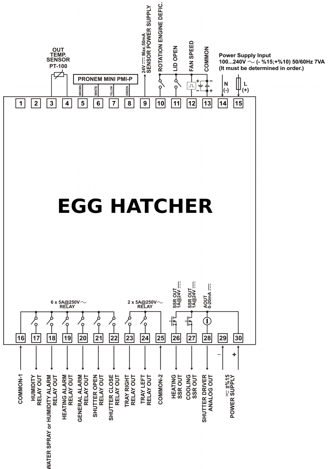
Electrical Wiring Diagram for Pronem Type Input Card
