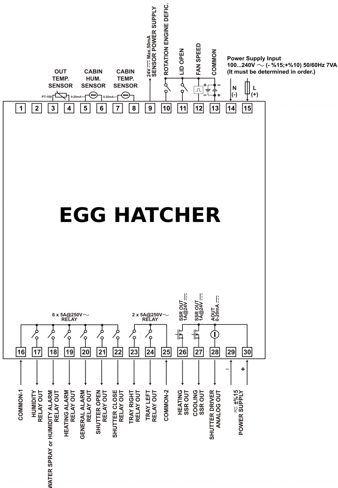
Electrical Wiring Diagram for mA Type Input Card
